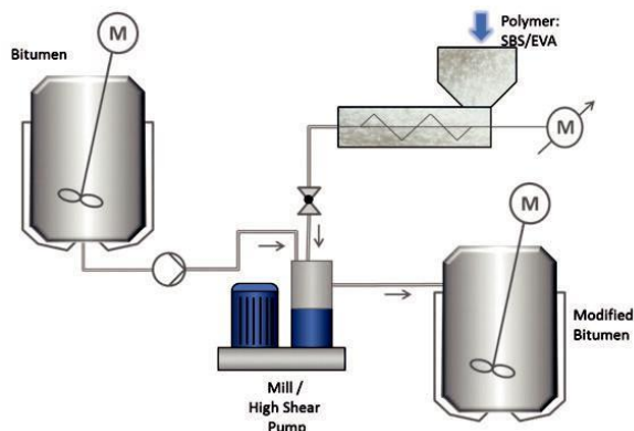
Figure 10: Typical mixing process of SBS and EVA modified bitumen
