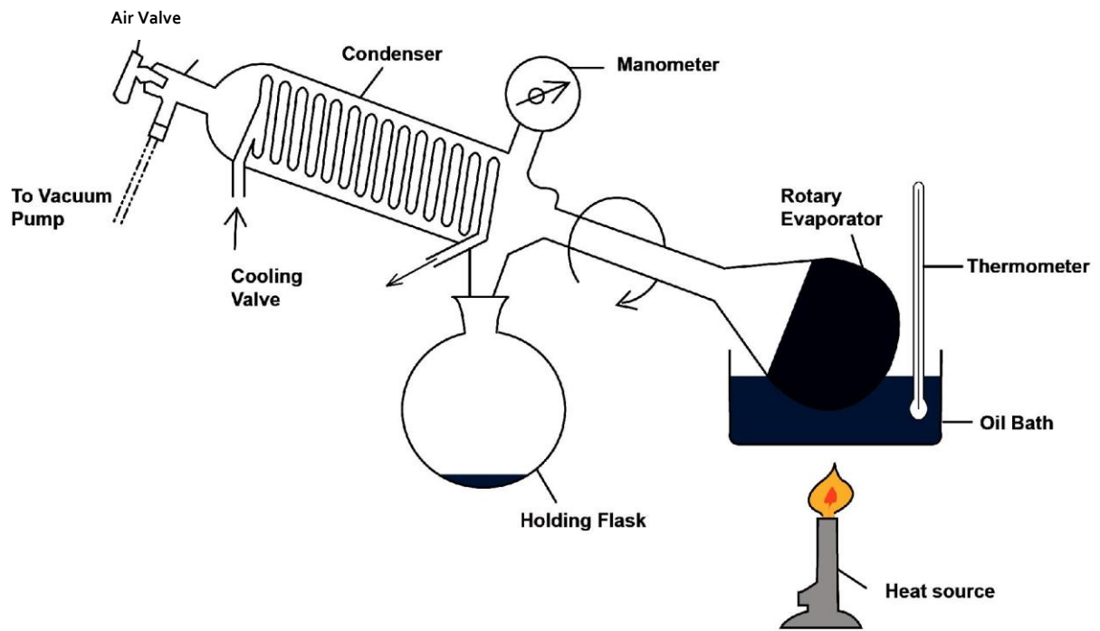
Figure 1: Preparation of polymer modified binder samples
