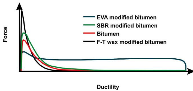
Figure 6: Typical force-ductility curves for various modified binders
