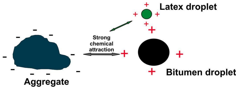
Figure 7 Adhesion characteristics of latex modified emulsions
