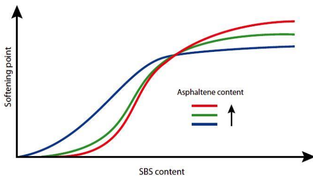
Figure 2: Typical effect of SBS on the softening point of bitumen with different asphaltene contents
