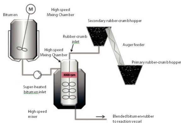
Figure 11: Schematic of a typical high speed bitumen-rubber blender
