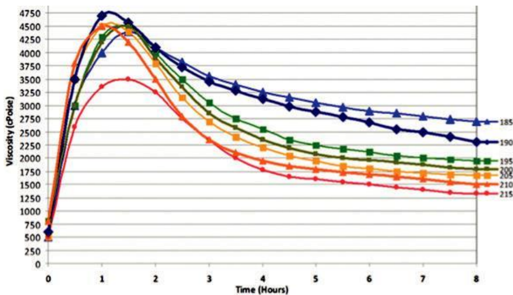
Figure 13: Typical changes in viscosity values for bitumen rubber at different temperatures over time
