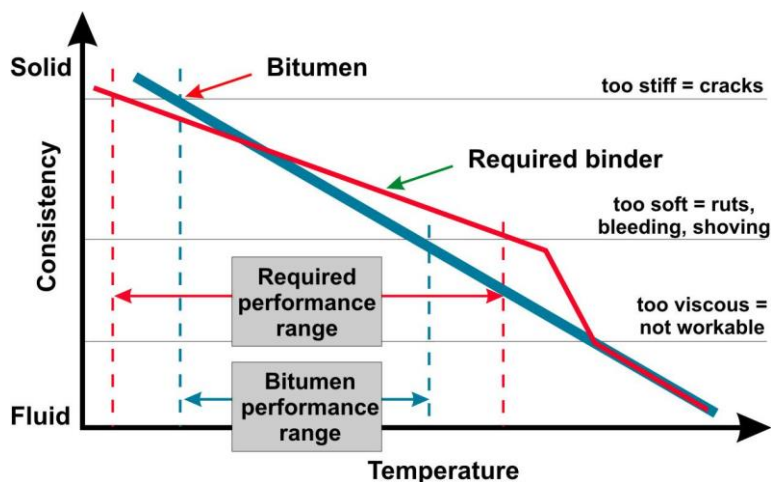
Figure 8: Schematic of viscosity of a binder over its working temperature range
