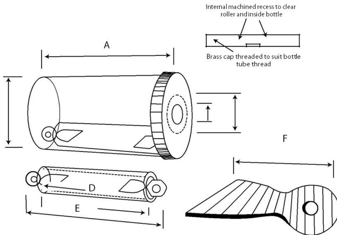
Figure 1: Metal treatment bottles and rollers
