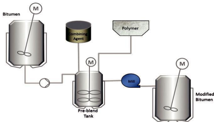
Figure 9: General production process of polymer modified bitumen
