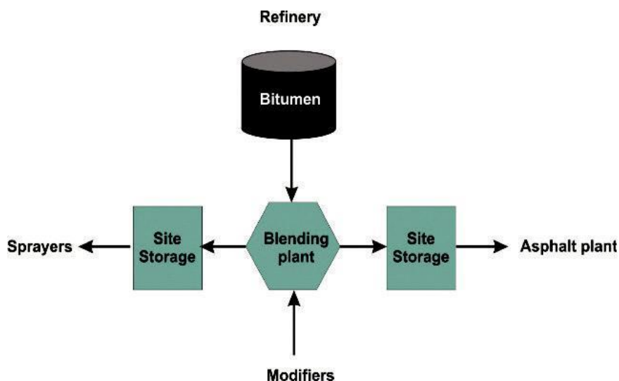
Figure 12: Process flow for handling modified binders
